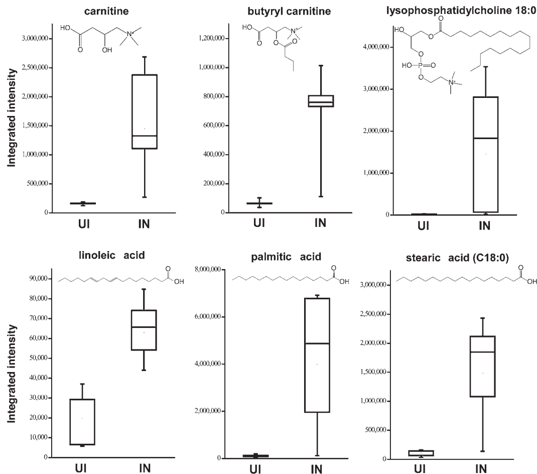
Figure 3 Box-and-whisker plots showing integrated intensities for selected ions in uninfected (UI) versus infected (IN) CSF, and proposed structures of the metabolites. Bottom and top of the boxes indicate 25th and 75th percentiles, and whiskers indicate 5th and 95th percentiles.
