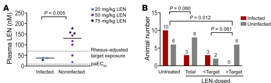
Figure 4. Animal infection status relative to LENO exposure at the time of challenge. (A) Plasma levels of LENO measured by mass spectrometry among SHIV-challenged animals at the time of challenge versus final infection status. Symbols represent plasma LENO concentration derived from an average of 3 biological assay replicates for individual study animals and are color-coded by the corresponding LENO-dosing groups. The horizontal bars represent group averages. The P value comparing exposures among infected versus uninfected animals, computed via an unpaired t test with Welch's correction, is shown. The lower dotted line represents the rhesus paEC_{95} for LENO (8.8 nM), while the higher dotted line represents the rhesus-adjusted clinical target C_{trough} concentration for LENO (70 nM). (B) Infection rates among the different study animal subgroups. Bars represent the number of infected (red) or uninfected (gray) study animals that were not treated, the total number of animals dosed with LENO or dosed with LENO and split into subsets with exposures below or above the adjusted LENO target concentration. P values, computed via Fisher's exact test, are shown.
